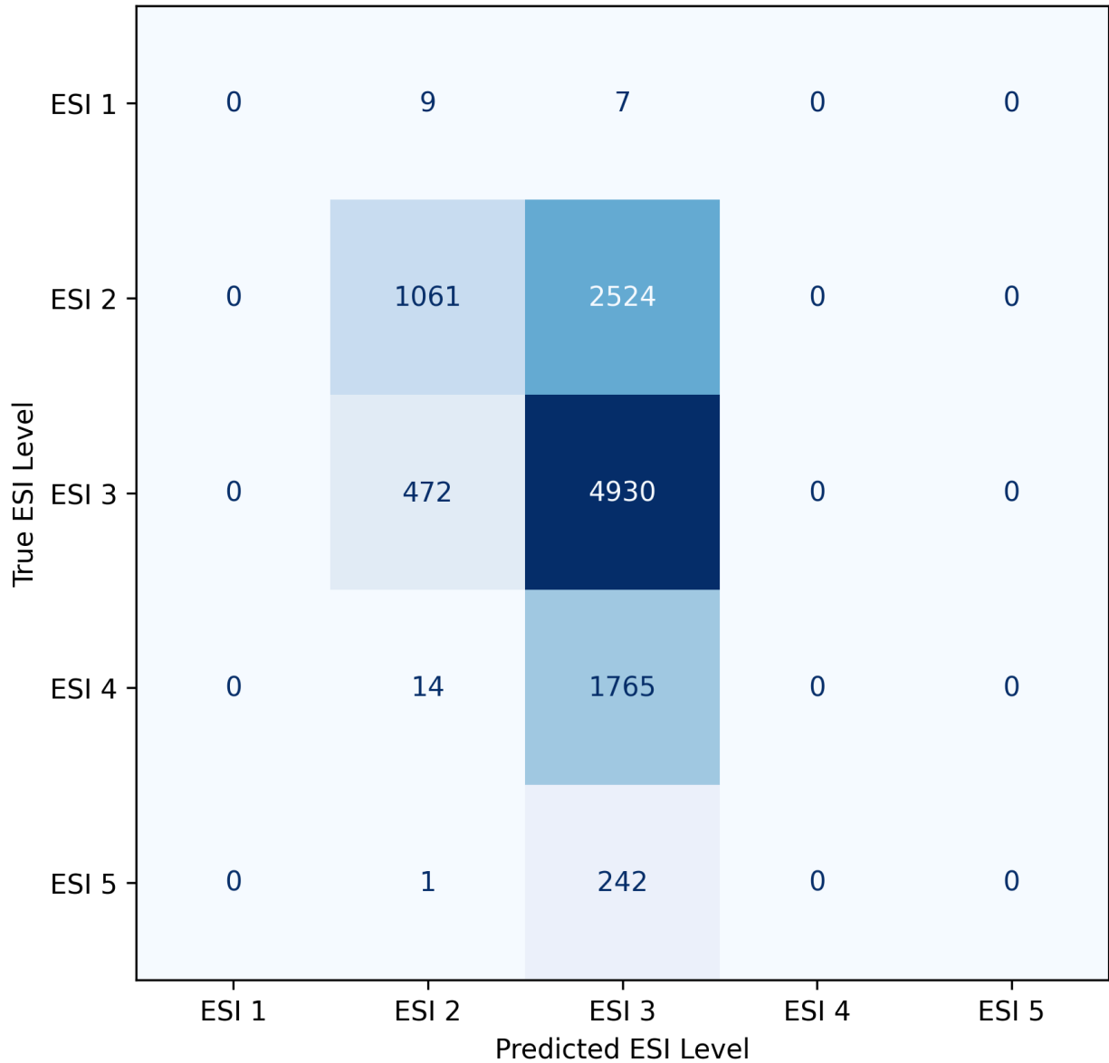
Decision Tree Confusion Matrix
